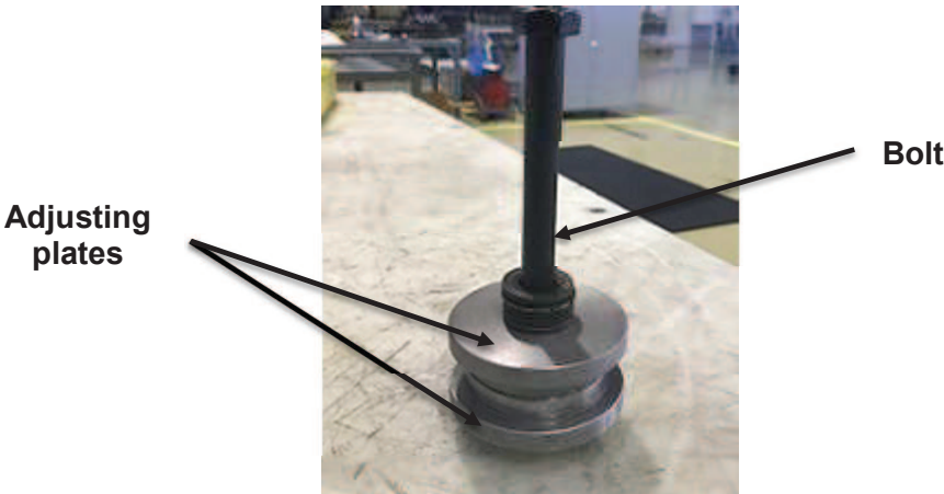
Picture 1. The 773 Transfer Gear Adjusting Fixture AS
